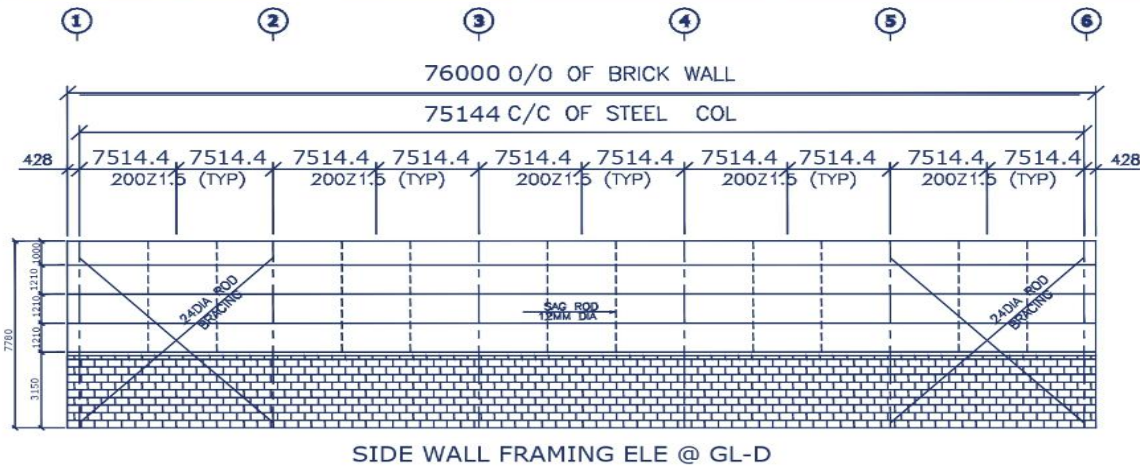
SIDE WALL FRAMING ELE @ GL-D
