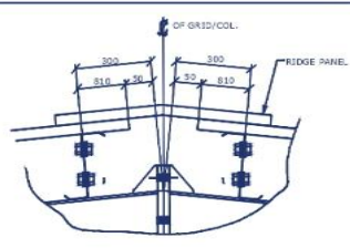
TYP. DETAIL OF RIDGE SAG ROD
