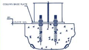
SECTIONAL VIEW - 2 BOLTS IN A ROW
