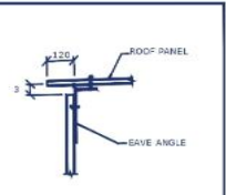
EAVE SHEET DETAILS
