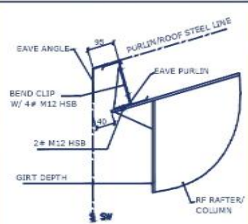
EAVE PURLIN CONNECTION (LOW SIDE EAVE)
